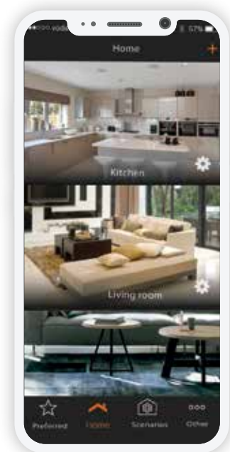
App MyHOME_Up
